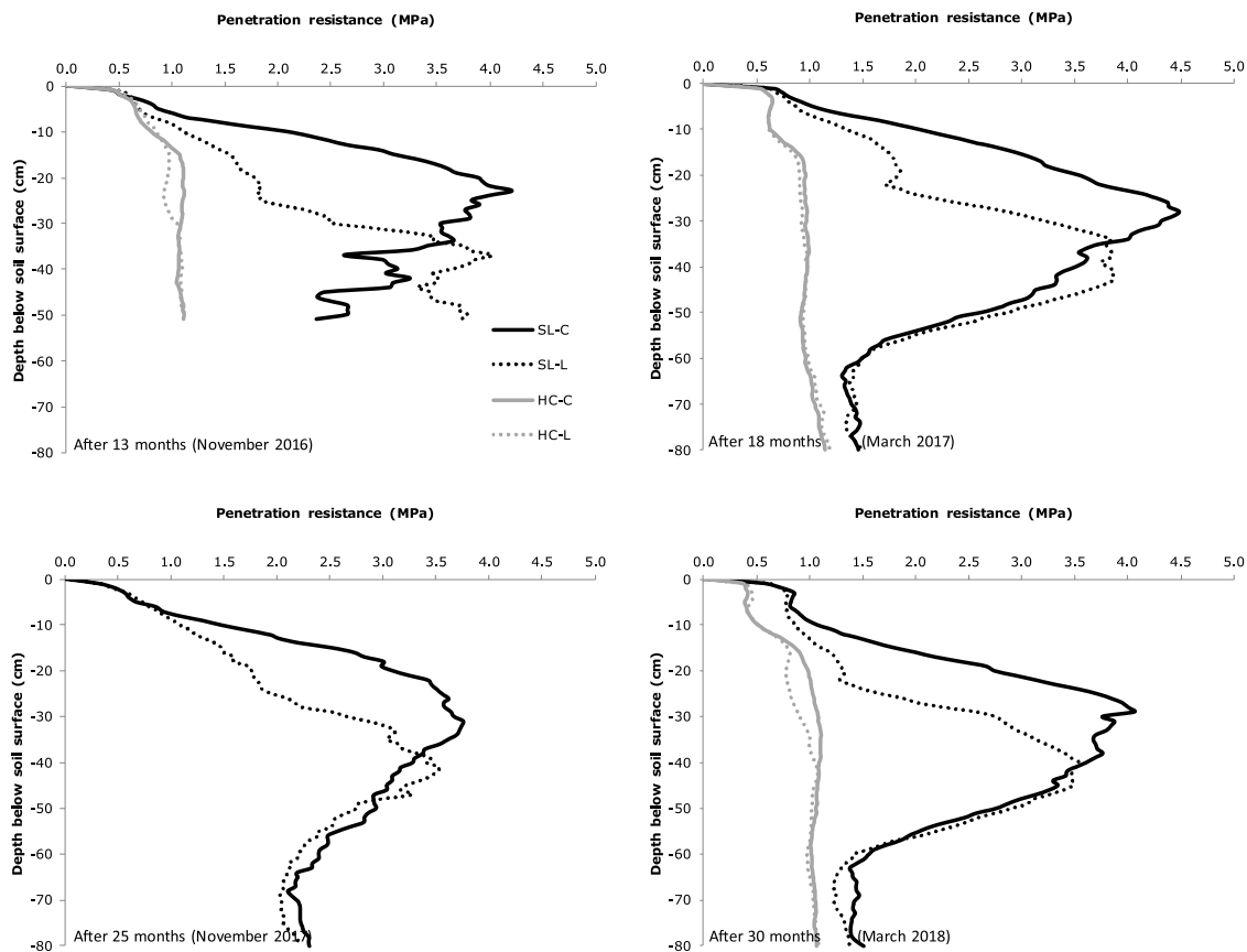
Fig. 1. Penetration resistance (MPa) in the 0–80 cm soil profile of compacted grassland on a sandy loam (SL) and heavy clay (HC), as influenced by sward lifting (L) and compared to the untreated control (C). Measurements were 13, 18, 25, and 30 months after treatment in the autumn of 2015. Results for heavy clay after 25 months are not reported, because a methodological error was made during measurement.
