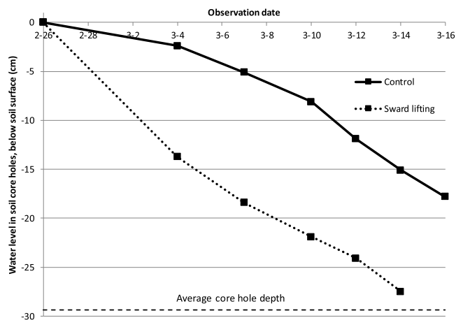
Fig. 2. Decline in the water level of initially water-filled soil core holes in grassland on a heavily compacted sandy loam, as influenced by sward lifting and compared to the control treatment, measured in early spring 2017. The decline in water level over time is used as a proxy for water drainage rate.
